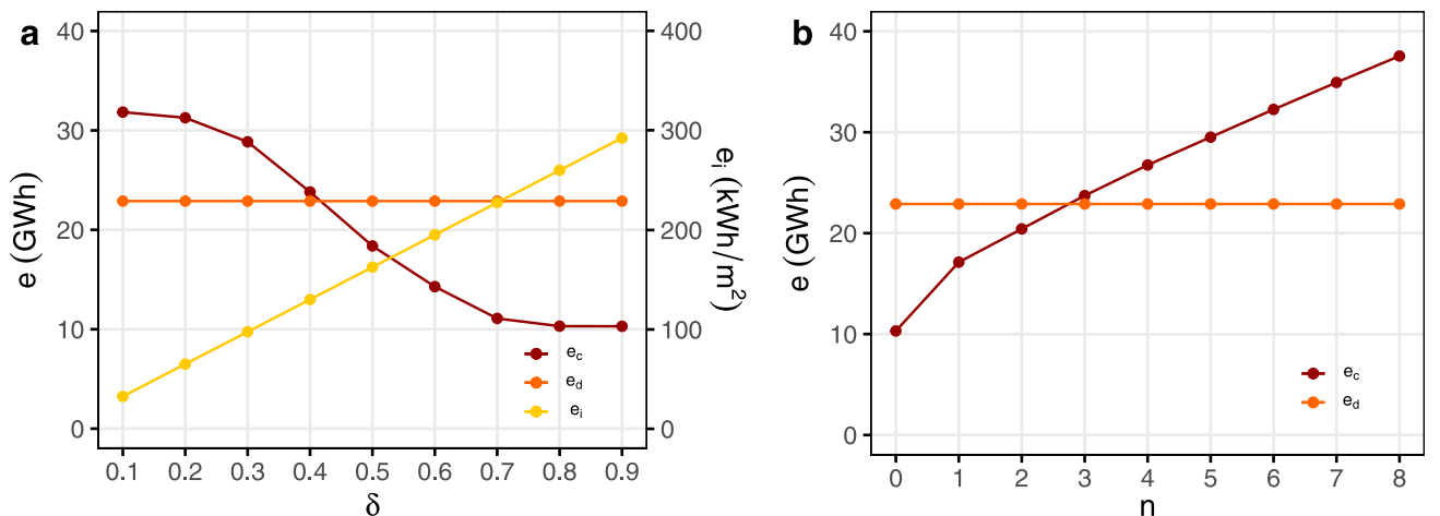
Fig. 8. Availability of solar PV potential. (a) The total solar PV potential when utilizing a series of solar PV intensities. (b) The total solar PV potential when utilizing a number of additional rooftops.
